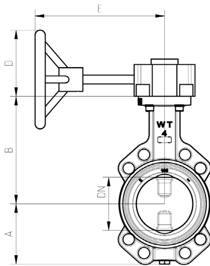
Type ZF
